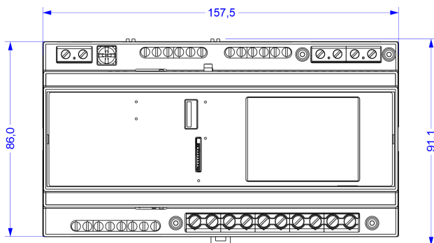
Fig. 4. Analyzer's external dimensions (in millimeters).
