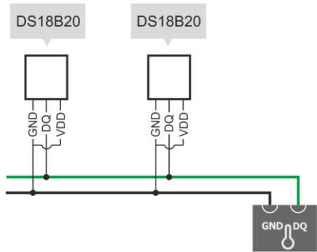
Fig. 33. Connection of 1-Wire sensors to PQM-750 analyzer.
